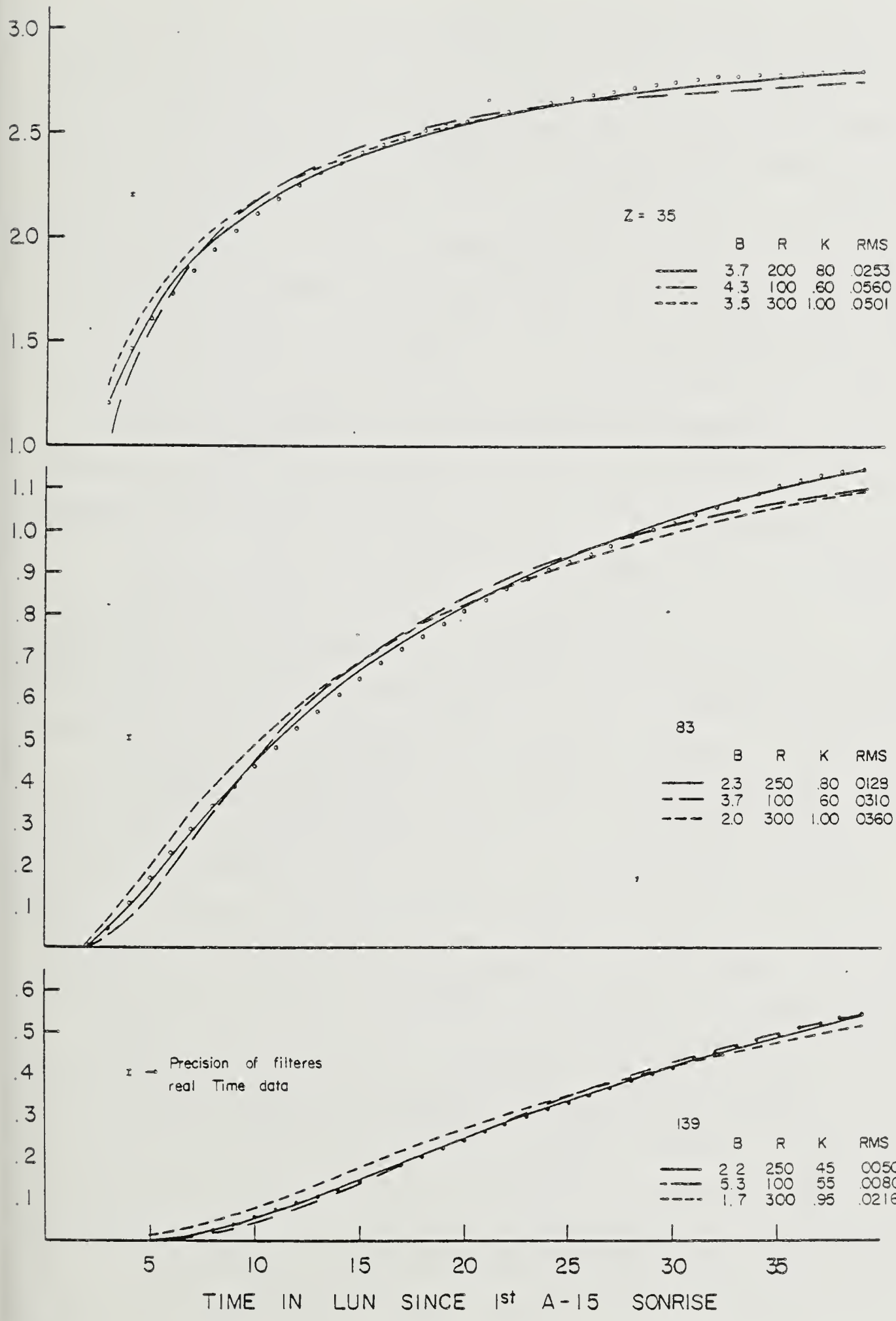
its to the astronaut induced transient component at representative A-15 sensors
